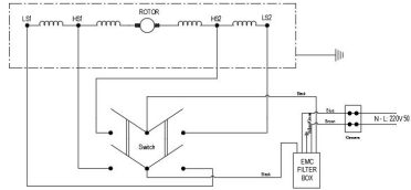
MOTOR CONNECTION WITH EMC FILTER
