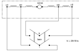
MOTOR CONNECTION WITHOUT EMC FILTER
